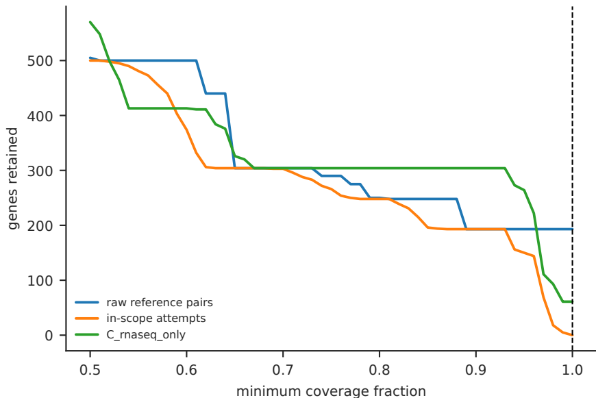
Coverage gate sweep
