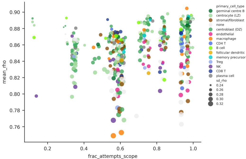
Coverage vs behaviour (point size = SD of \rho )
