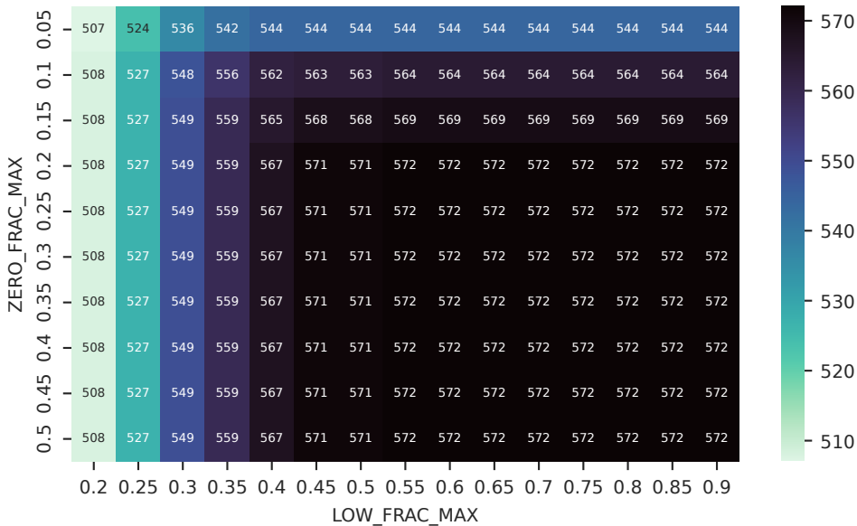
Genes surviving the QC gate
