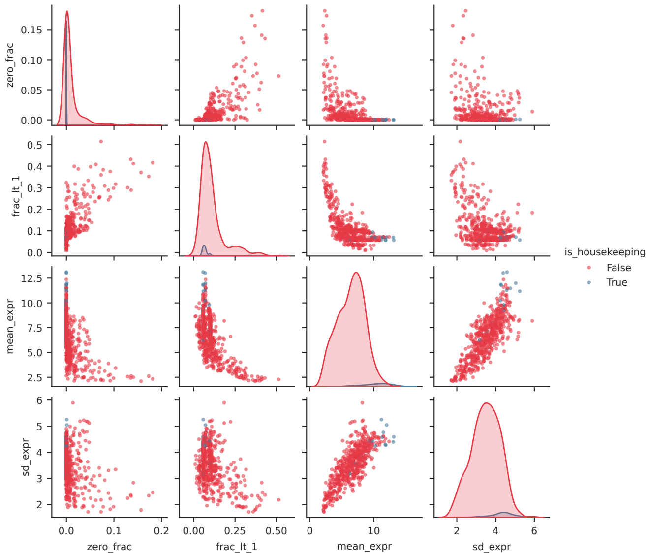
Expression QC statistics (01_raw)
