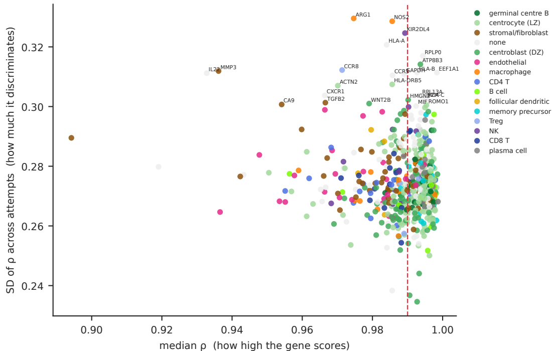
Discriminative power: the y axis is what selection maximises
