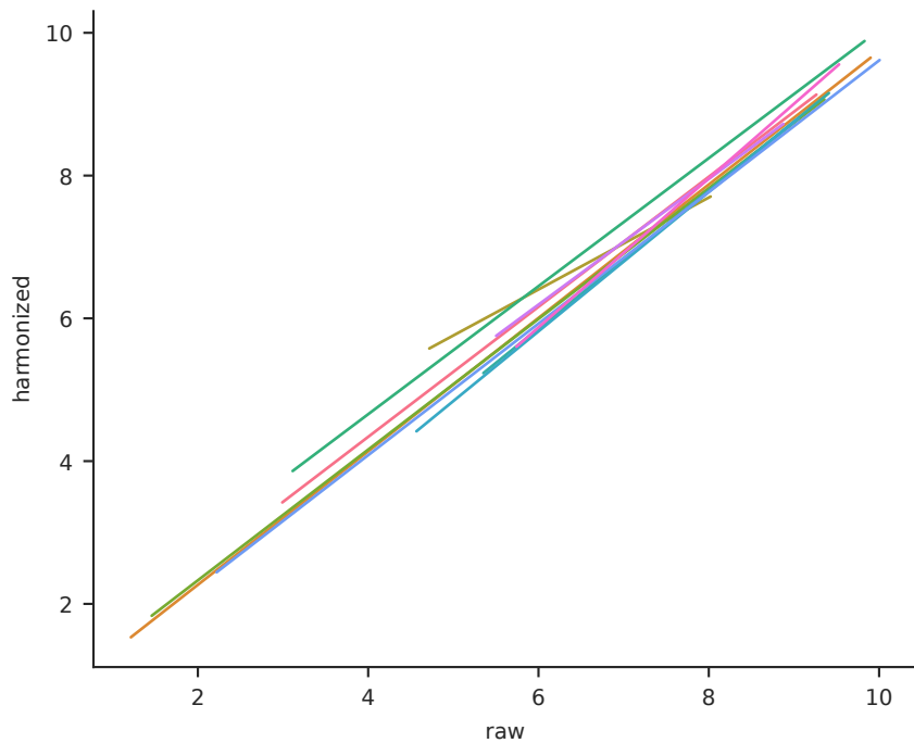
CNN2: per-cohort regression lines mean within-cohort \rho = 0.945
