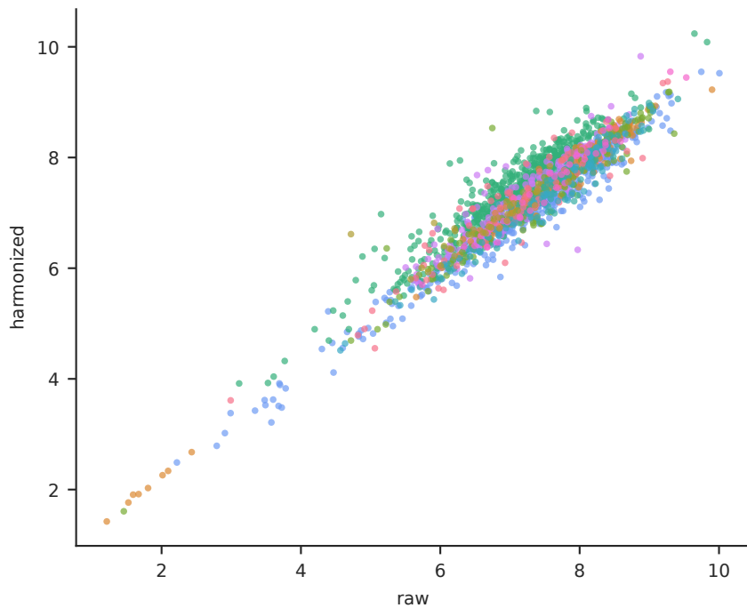
CNN2: all cohorts pooled pooled \rho = 0.907
