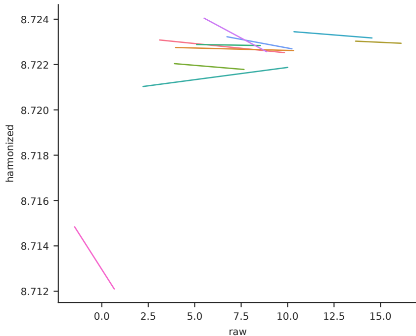
CNN2: per-cohort regression lines mean within-cohort \rho = -0.125
