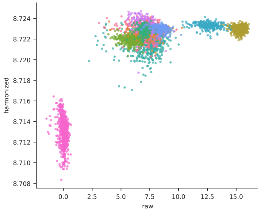
CNN2: all cohorts pooled pooled \rho = 0.628
