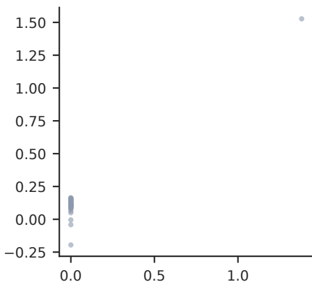
PDGFC · PUB_Beguelin worst \rho = -0.327
