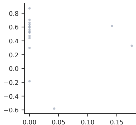
PGF · PUB_Health_B worst \rho = 0.408
