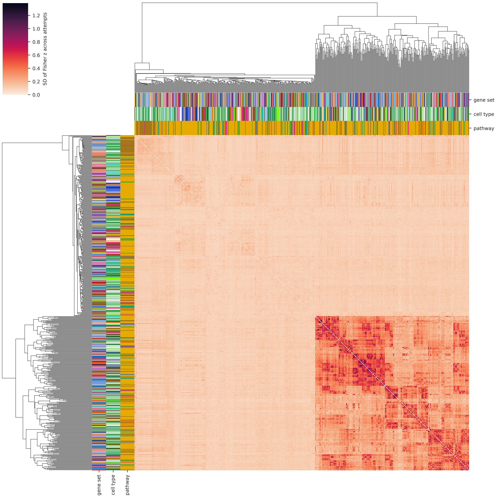
Stability of each gene-gene relationship
