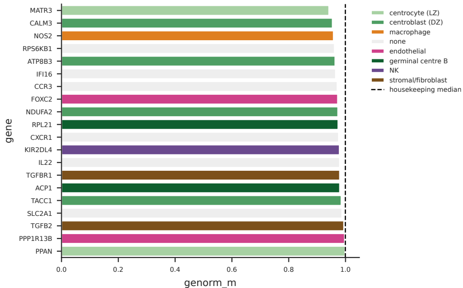
20 most stable marker genes
