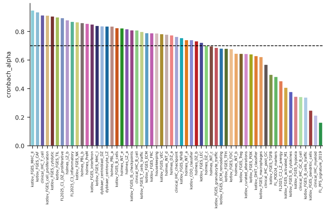
Cronbach's \alpha per signature (0.7 = conventional adequacy)
