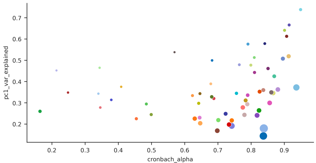
Coherence: \alpha vs PC1 variance explained
