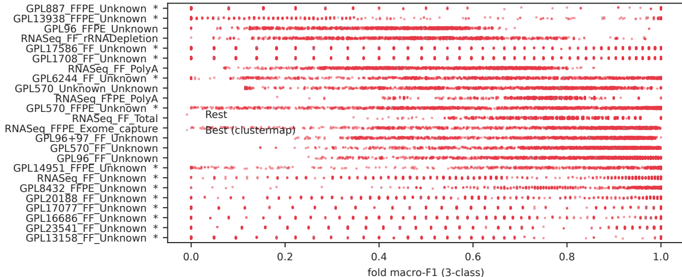
Per-batch difficulty (* = single-class batch, no AUC)
