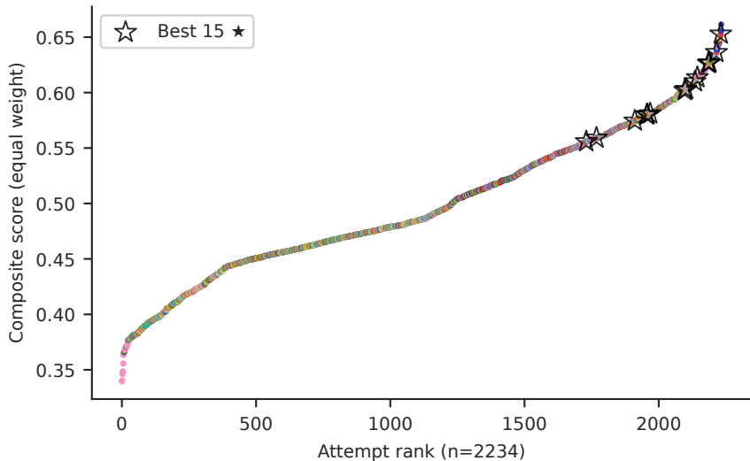
A: Ranking of all harmonization attempts — Best 15 ★ concentrated in top percentile
