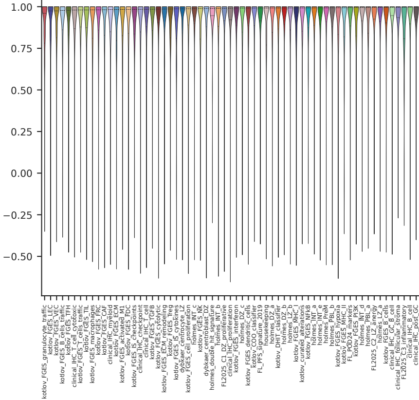
p distribution per gene set (primary membership)
