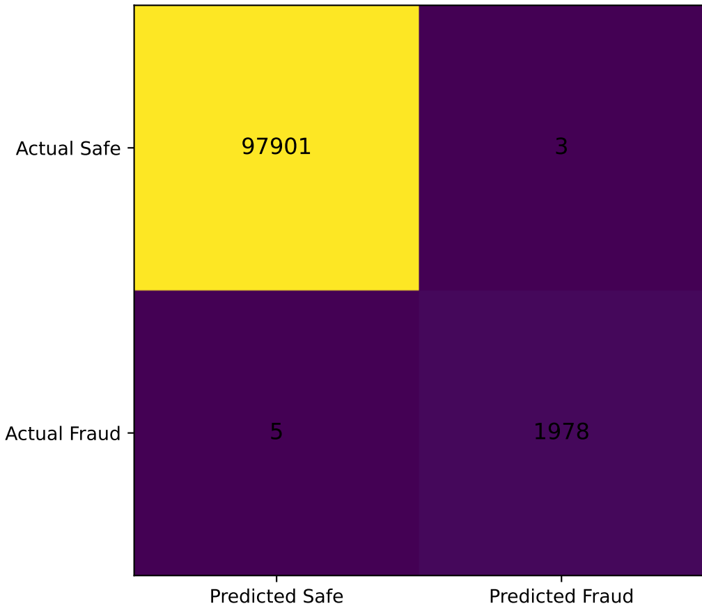
LightGBM Confusion Matrix
