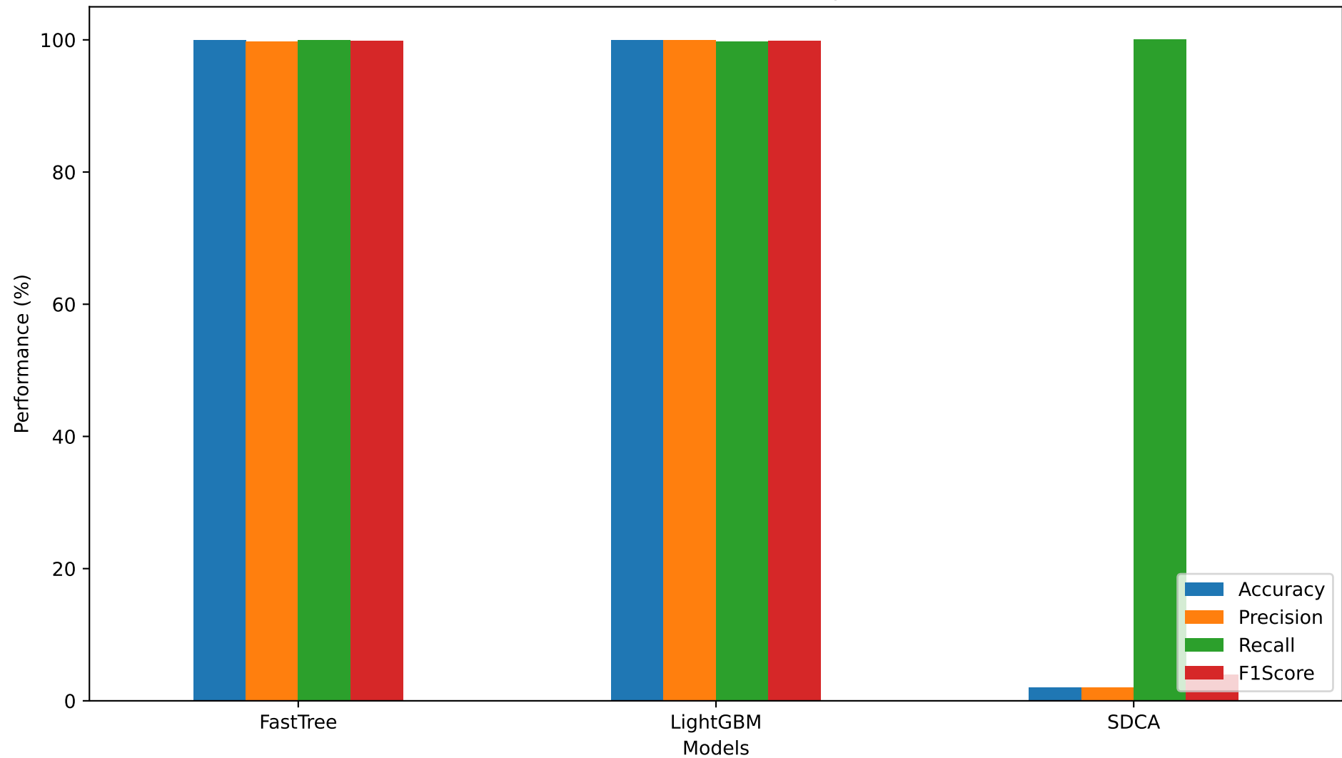
Fraud Detection Model Comparison
