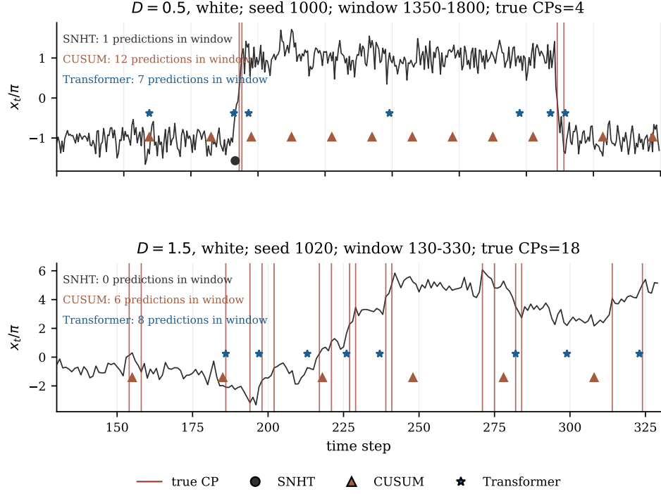
Fig. 5. Representative detection windows. Vertical lines show true change points; markers show selected method predictions.
