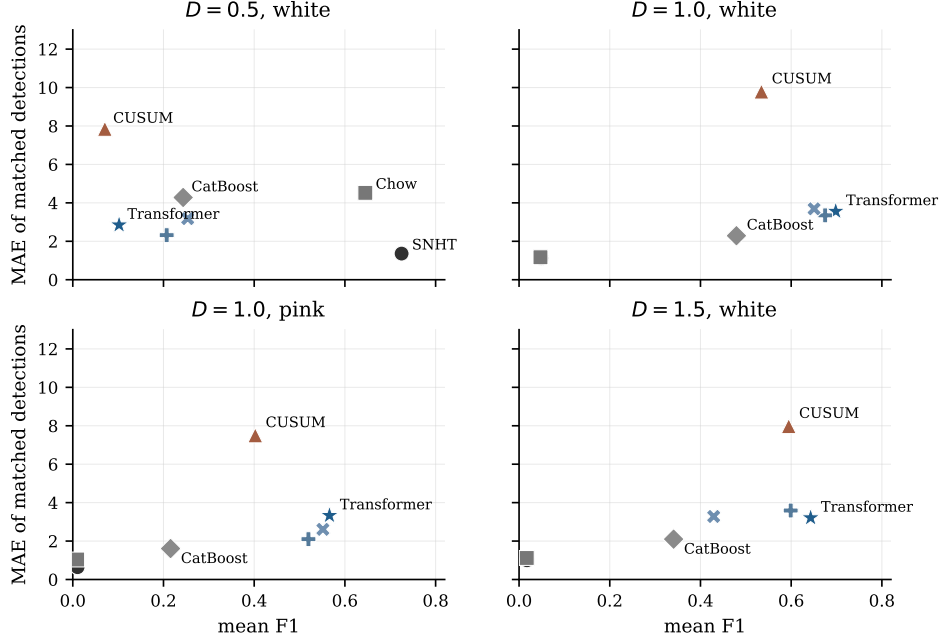
Fig. 4. Mean F1 and mean absolute localization error for selected methods at the primary matching margin. MAE is computed only for matched detections and should be read together with F1.
