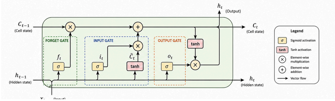
Figure 2: Gated information flow through an LSTM cell, showing the forget, input and output gates, candidate memory, cell state and hidden state. Redrawn for this report from the standard LSTM formulation [12].
