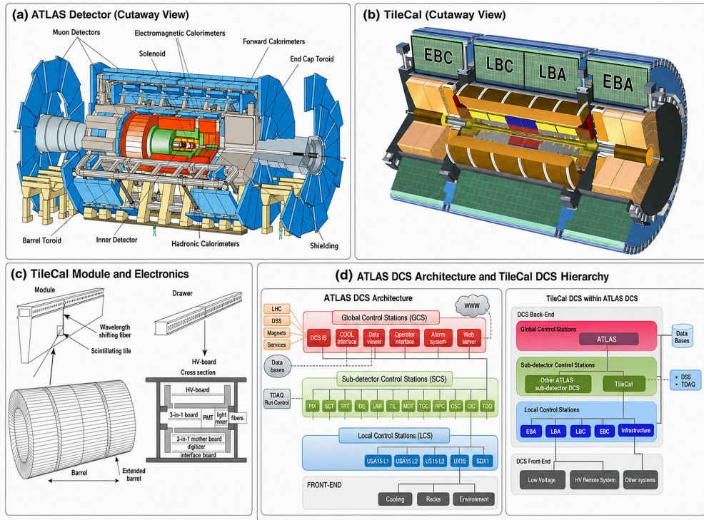
Figure 1: Detector and control-system context for the study: ATLAS, the four TileCal read-out partitions, representative module electronics, and the relationship between the ATLAS-wide DCS and TileCal DCS. Source images are adapted from ATLAS/TileCal/DCS documentation and the source MSc study [8, 9, 10, 15].
