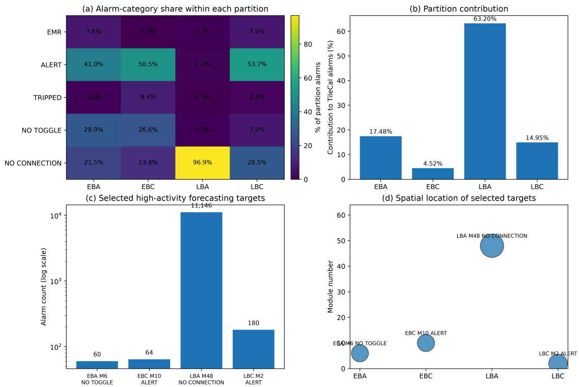
Figure 4: Spatial alarm activity and high-activity forecasting targets derived from the source analysis [15].
