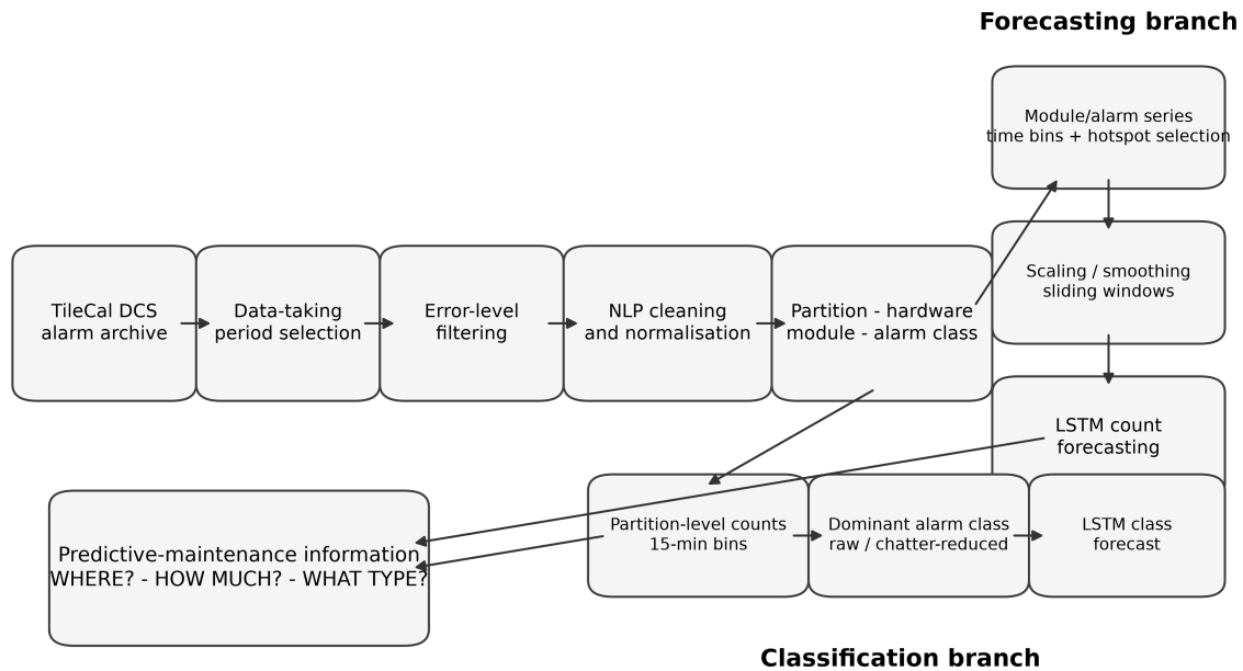
Figure 3: End-to-end TileCal alarm-analysis workflow, from DCS records and NLP extraction to module-level forecasting, partition-level classification and predictive-maintenance outputs.
