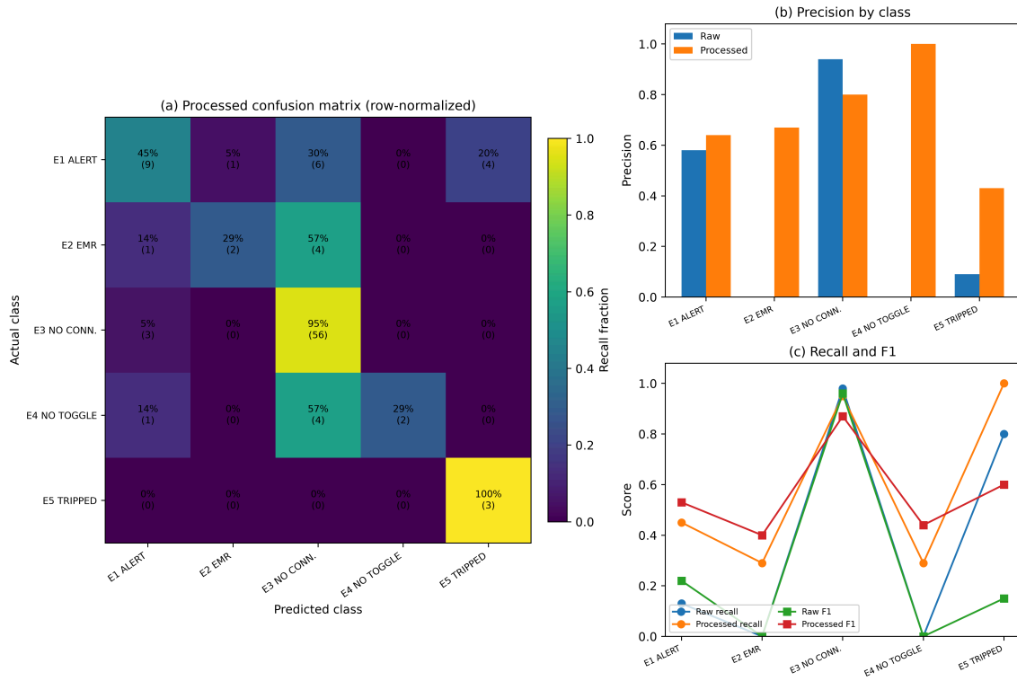
Figure 6: Effect of chattering reduction on dominant alarm-type classification: processed confusion matrix and raw-versus-processed class-level precision, recall and F1.
