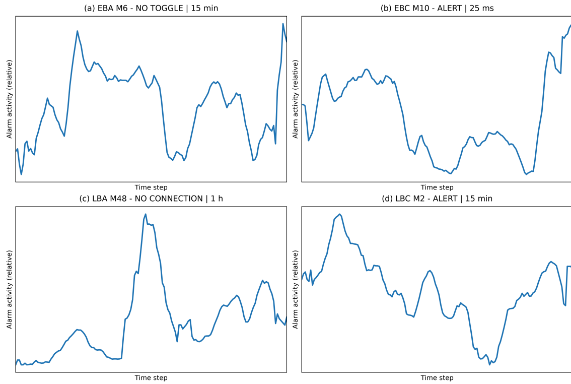
Figure 5: Temporal behaviour of the four selected module-alarm series at their final modelling resolutions: 15 min (EBA), 25 ms (EBC), 1 h (LBA) and 15 min (LBC).
