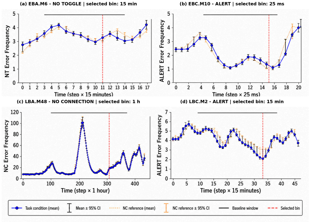
Figure 5: Temporal behaviour of the four selected module-alarm series at their final modelling resolutions: 15 min (EBA), 25 ms (EBC), 1 h (LBA) and 15 min (LBC).
