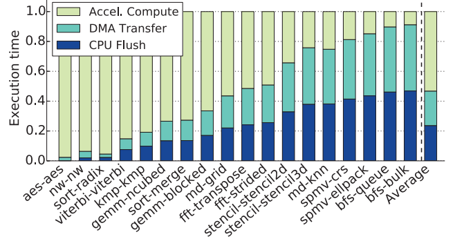
(b) Breakdown of flush, DMA, and compute time in MachSuite for 16-way parallel designs.
