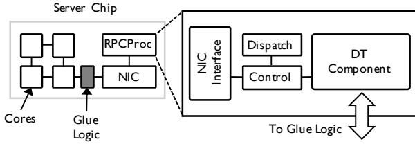
Figure 4: Architecture of an on-chip RPC processor.
