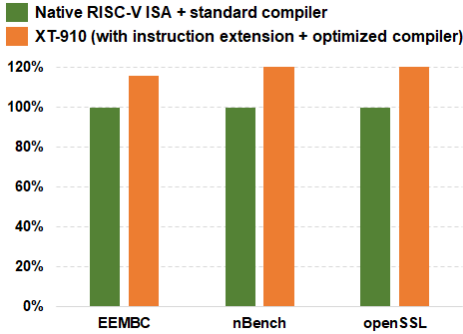
Fig. 20: The performance of XT-910 with instruction extensions and optimized compiler, normalized to using native RISC-V ISA and compiler.
