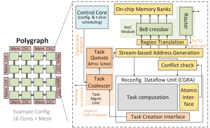
Fig. 11: PolyGraph Modular Hardware Implementation
