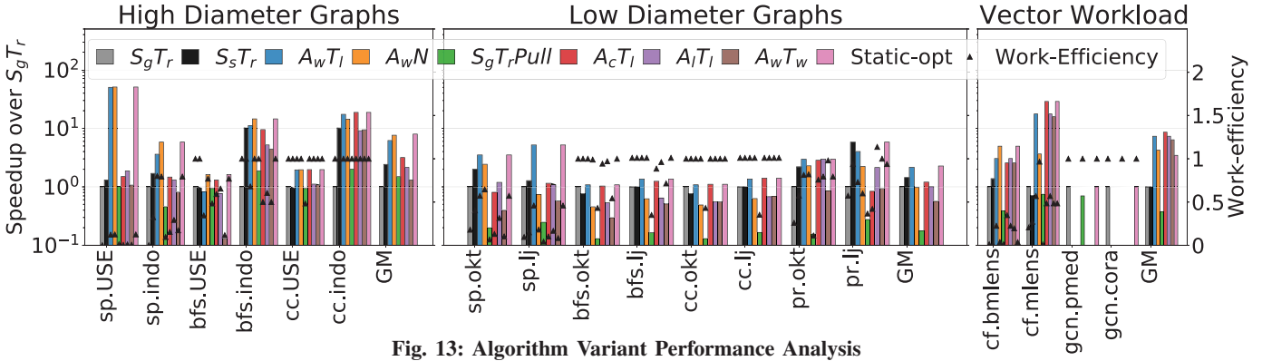
Fig. 13: Algorithm Variant Performance Analysis
