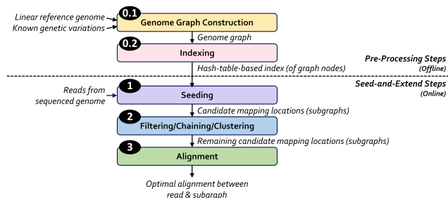
Figure 2: Sequence-to-graph mapping pipeline.
