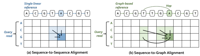
Figure 3: Data dependencies in (a) sequence-to-sequence alignment, and (b) sequence-to-graph alignment.
