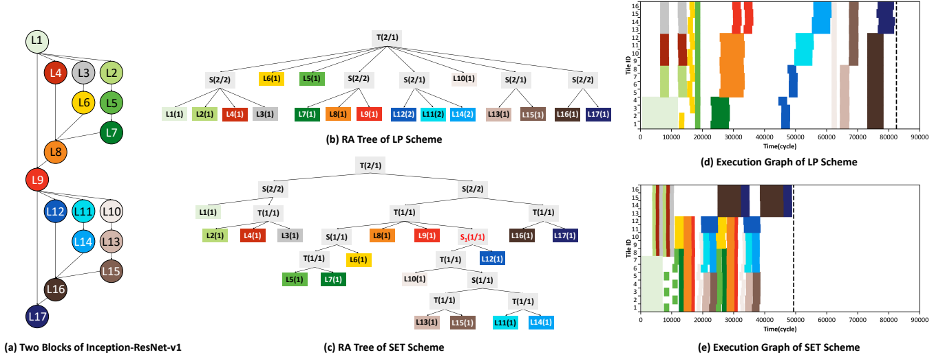
Figure 5: A practical comparison of two schemes: one explored within the space defined by our RA Trees (abbreviated as SET scheme), and the other explored by Tangram-like strategy [17], which mainly falls in LP pattern (abbreviated as LP scheme). The practical execution graph of both RA Trees are drawn by the cycle-accurate simulator of a 16-tile accelerator.
