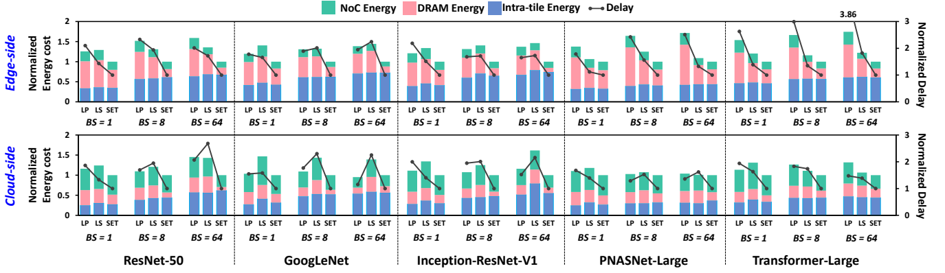
Figure 8: Comparisons among LP, LS, and SET with different batch sizes (BS), workloads, and hardware platforms. Each row takes the same platform, and each column takes the same workload.
