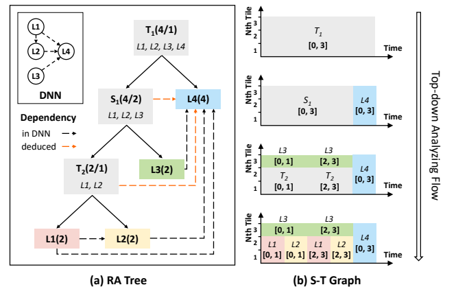
Figure 2: (a) An example RA Tree. (b) The top-down hierarchical analyzing flow of the left RA Tree. The bottom one is the S-T Graph corresponding to the left RA Tree. For simplicity, the dependencies of the RA Tree are only drawn in this figure.
