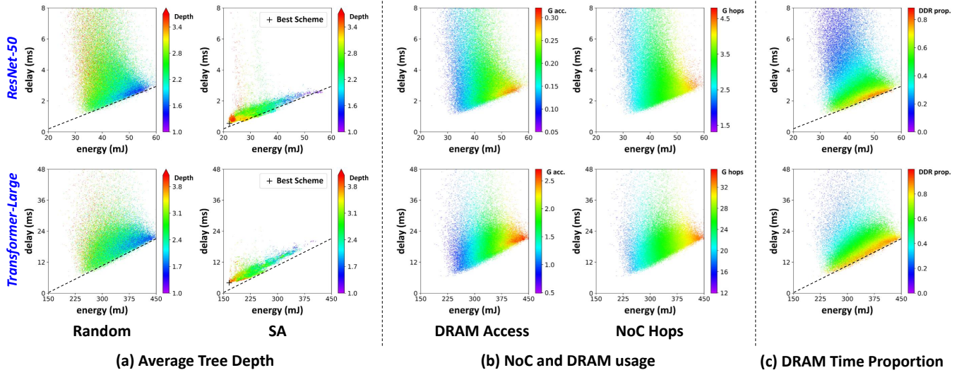
Figure 11: Scheduling space depiction. Each colored dot represents an RA Tree under the cloud platform and batch size 8. (a) The average tree depth of random RA Trees and RA Trees on the search path of SA. Depth is averaged among the depth of all Leaves. (b) The DRAM access and NoC hops of random RA Trees. (c) The proportion of DRAM time (defined in Sec. 6.1 (2)) over total delay of random RA Trees. All “RANDOM” figures show the same set of schemes, but exhibit different features.
