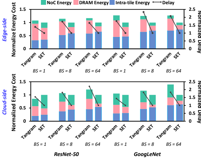
Figure 9: Comparison with Tangram
