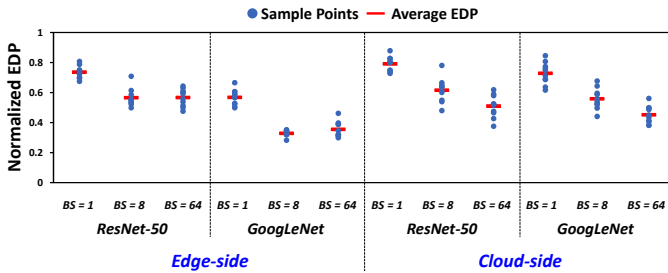
Figure 10: Variance of SET improvements. The SA algorithm is evaluated 10 times on each setting, and the EDP on each evaluation and their average are plotted above. The Y-axis is the normalized EDP, where the EDP of Tangram is normalized to 1.
