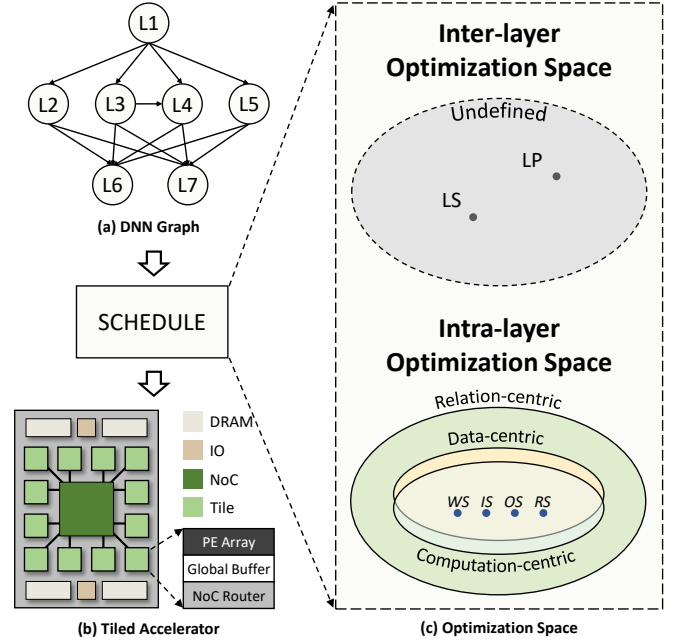
Figure 1: Left: The deploying flow from the DNN graph to the accelerator. Right: The two spaces for scheduling DNNs on the tiled accelerators, including undefined inter-layer scheduling space and well-defined intra-layer scheduling space (the inclusion relationship between the intra-layer scheduling spaces defined by different notations is drawn according to Tenet [37]).
