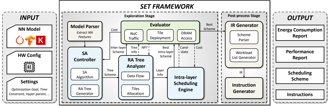
Figure 6: An overview of SET scheduling framework. Solid arrows represent the SA iteration loop, and dotted arrows represent local calls to the evaluator from each engine.
