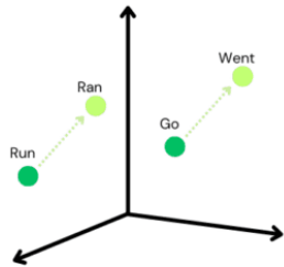
Verb Tense
