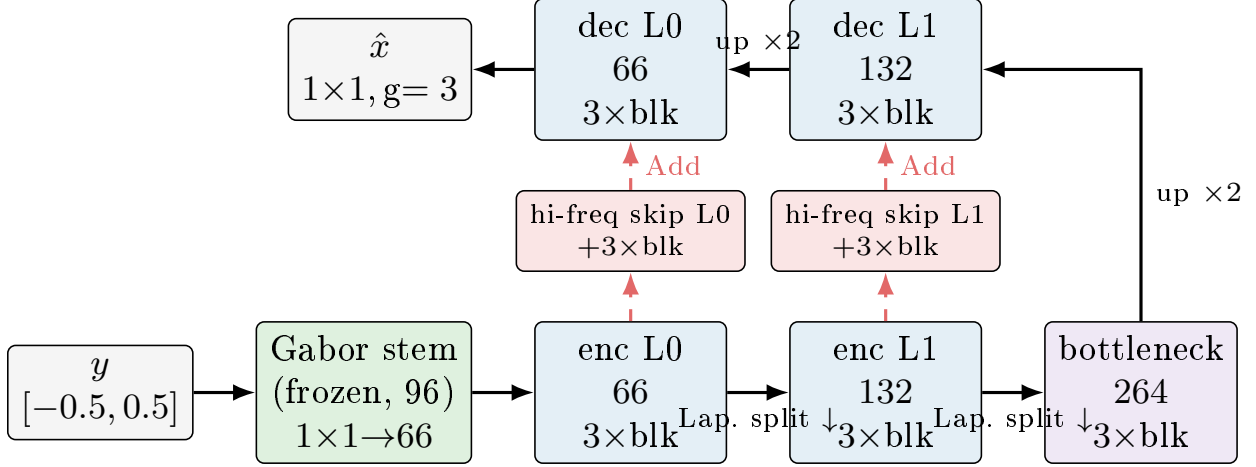
Figure 1: BF-CONVUNEXT data flow (channel widths shown). A frozen Gabor stem feeds a two-level CONVNEXT-V1 U-Net. Downsampling is a Laplacian-pyramid split: the low-frequency band descends (solid), the full-resolution high-frequency residual becomes the skip (dashed), passing through three extra bias-free CONVNEXT blocks before a parameter-free channel-matched Add into the decoder. The head is a bias-free grouped 1 \times 1 convolution (3 groups). Every operation is degree-1 homogeneous at inference.
