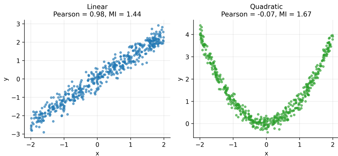
Figure 4: Mutual information vs. Pearson on a linear relationship (both informative) and a quadratic relationship (Pearson collapses to \approx 0 , MI remains high). MI characterises any form of statistical dependence, not just linear association.
