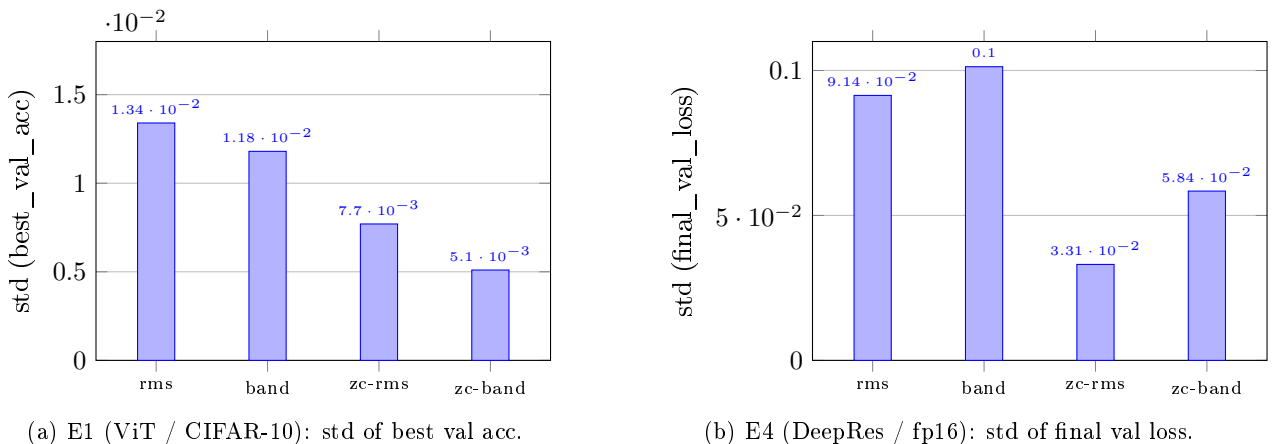
Figure 2: Seed-to-seed standard deviation across n=5 runs on E1 and E4. Zero-centered variants achieve 42%–64% lower std. The combined variant attains the lowest std on E1; pure ZEROCENTEREDRMSNORM attains the lowest on E4.
