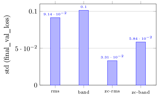
(b) E4 (DeepRes+fp16): seed std of final val loss.
