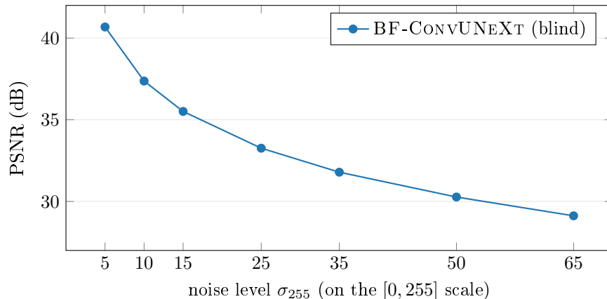
Figure 2: Blind PSNR vs. noise on DIV2K-validation (100 patches, 256px). One model spans \sigma_{255} \approx 5 –65 with no noise-level input. The 95% bootstrap CIs (not shown) are \pm 0.4 –0.8 dB.
