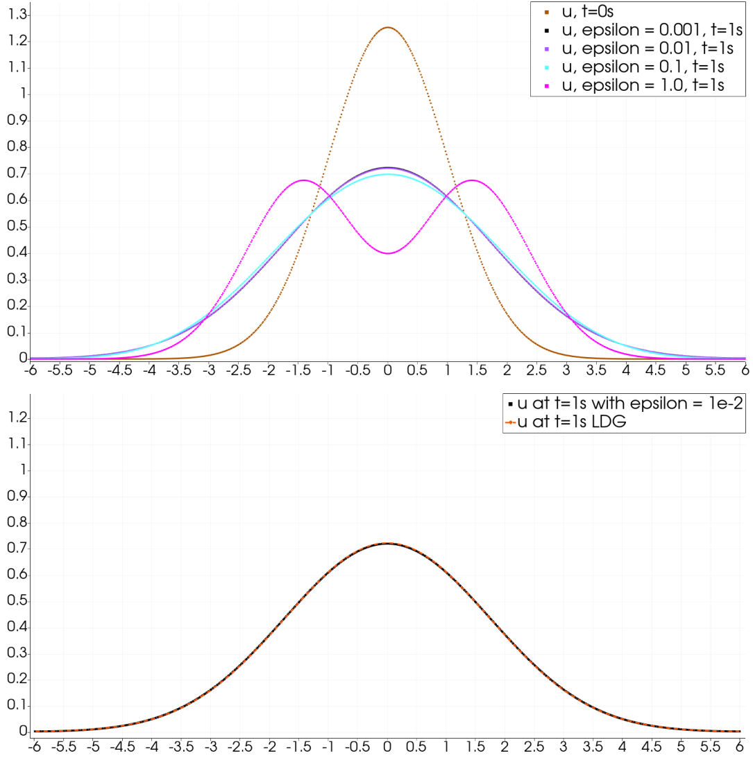
Fig. 5: Results for the hyperbolic system with varying \epsilon and a comparison to the LDGFE method for the exponent m = 1
