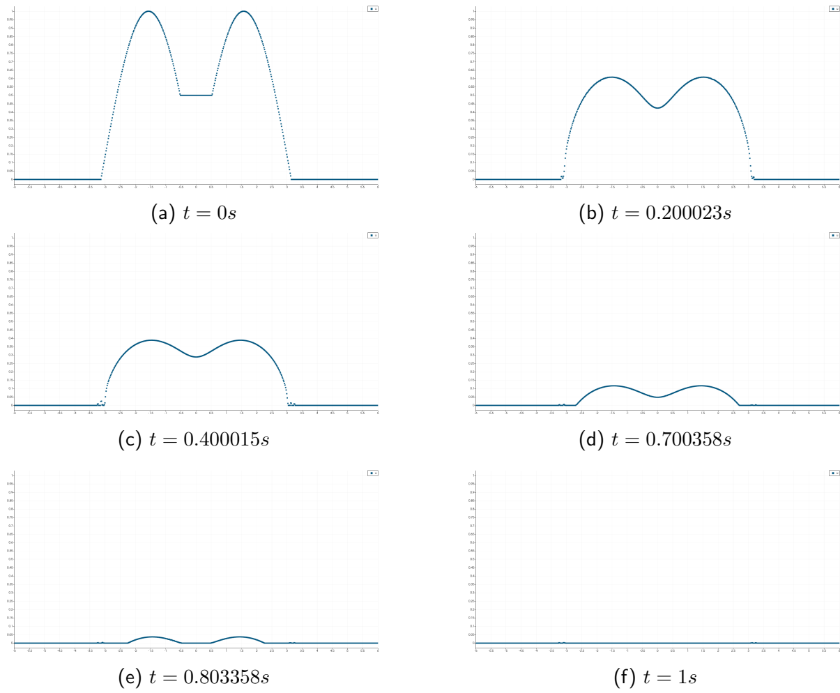
Fig. 10: Numerical results for the PME using the HBL system with strong absorption term with exponent p = 0.01 , m = 3 , c = 1 and polynomial degree l = 3
