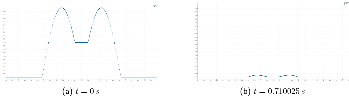
Fig. 11: Divorce of the support under enforcing the HBL system with parameters m = 1.98 and p = 0.02 . Calculated for N_{cells} = 320 and a polynomial degree of l = 2
