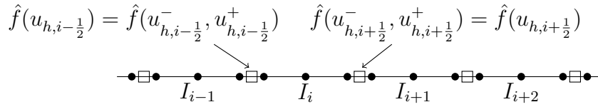
Fig. 1: Example cells with Gauss-Legendre nodes and interface fluxes for polynomial degree l = 3 .
