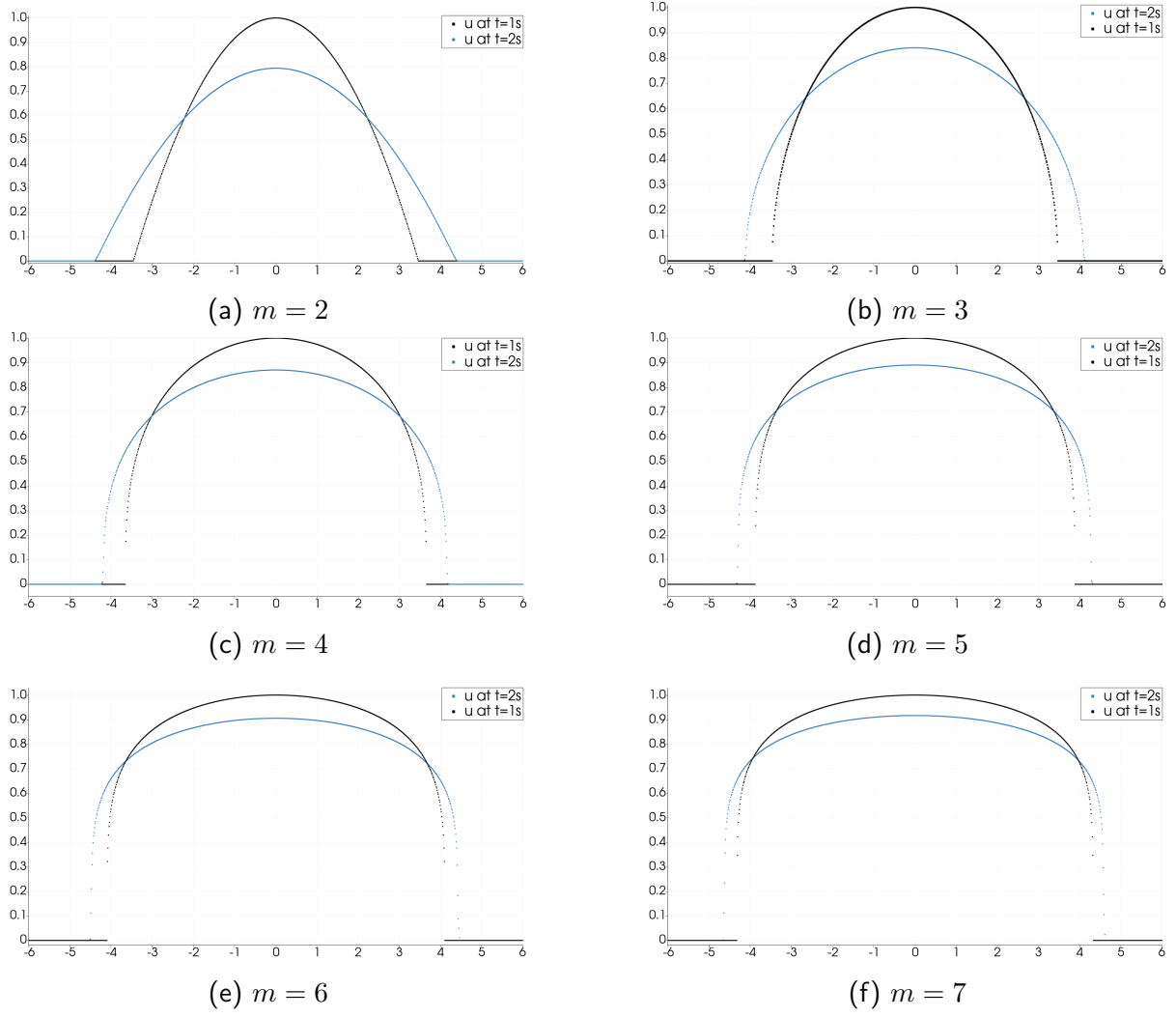
Fig. 3: Numerical results for the Barenblatt function as initial condition at t = 1s computed until the final time t = 2s . With the polynomial degree l = 3 and number of cells N_{cells} = 320 for various nonlinearities m .
