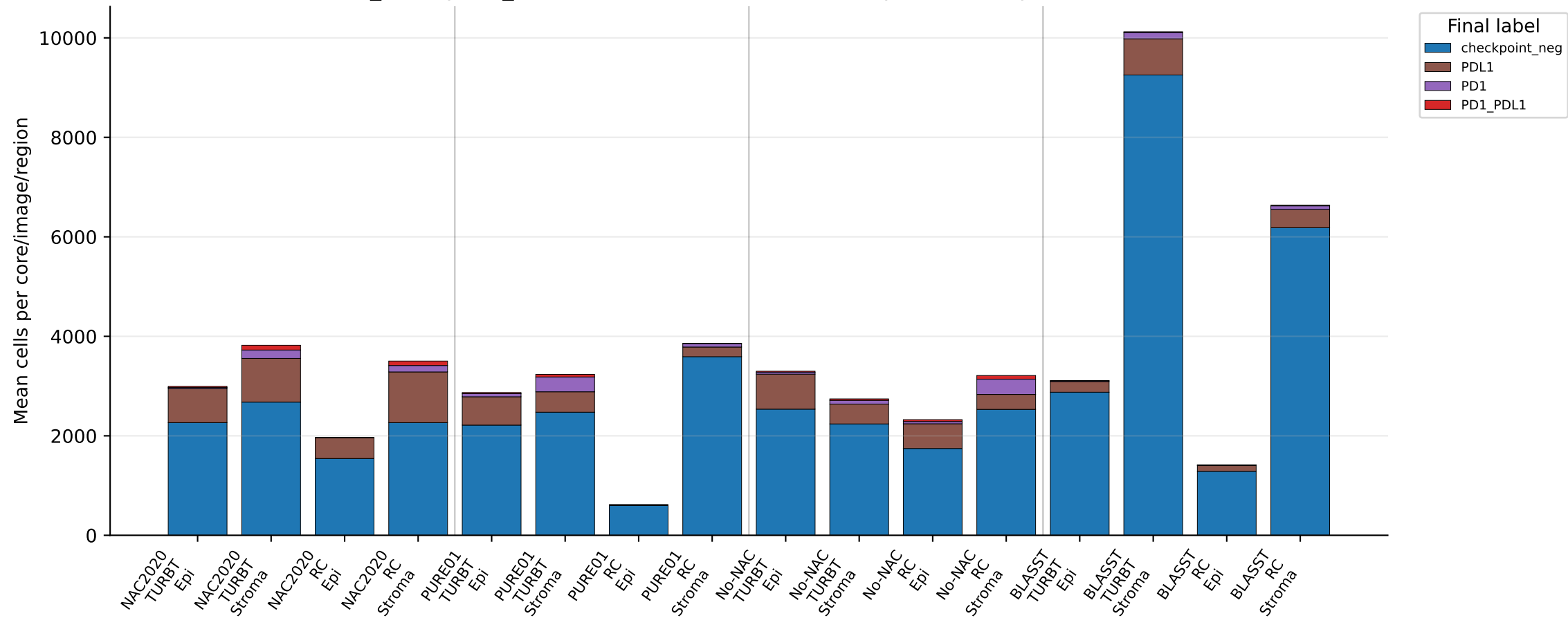
AR_checkpoint_state — AR: mean cell-count composition in Epi vs Stroma
