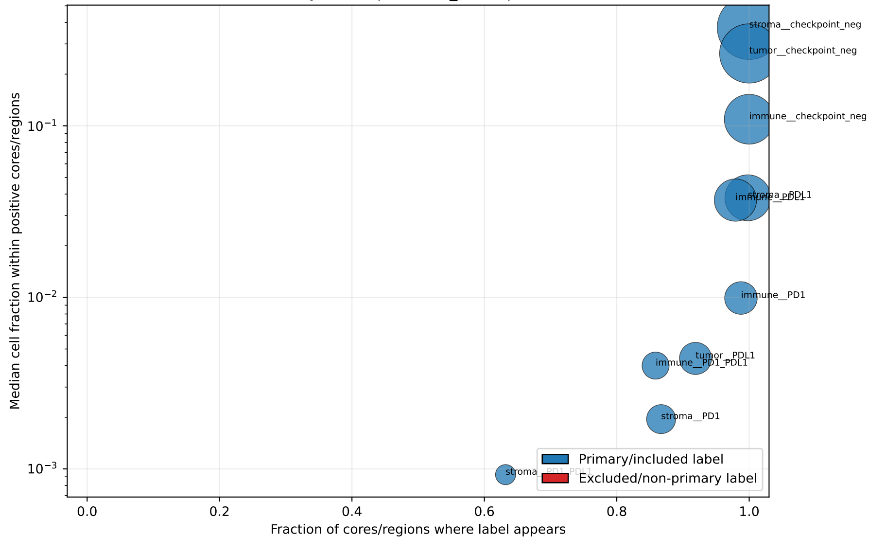
Abundance vs consistency — compartment_state, panel=AR (without BLASST)
