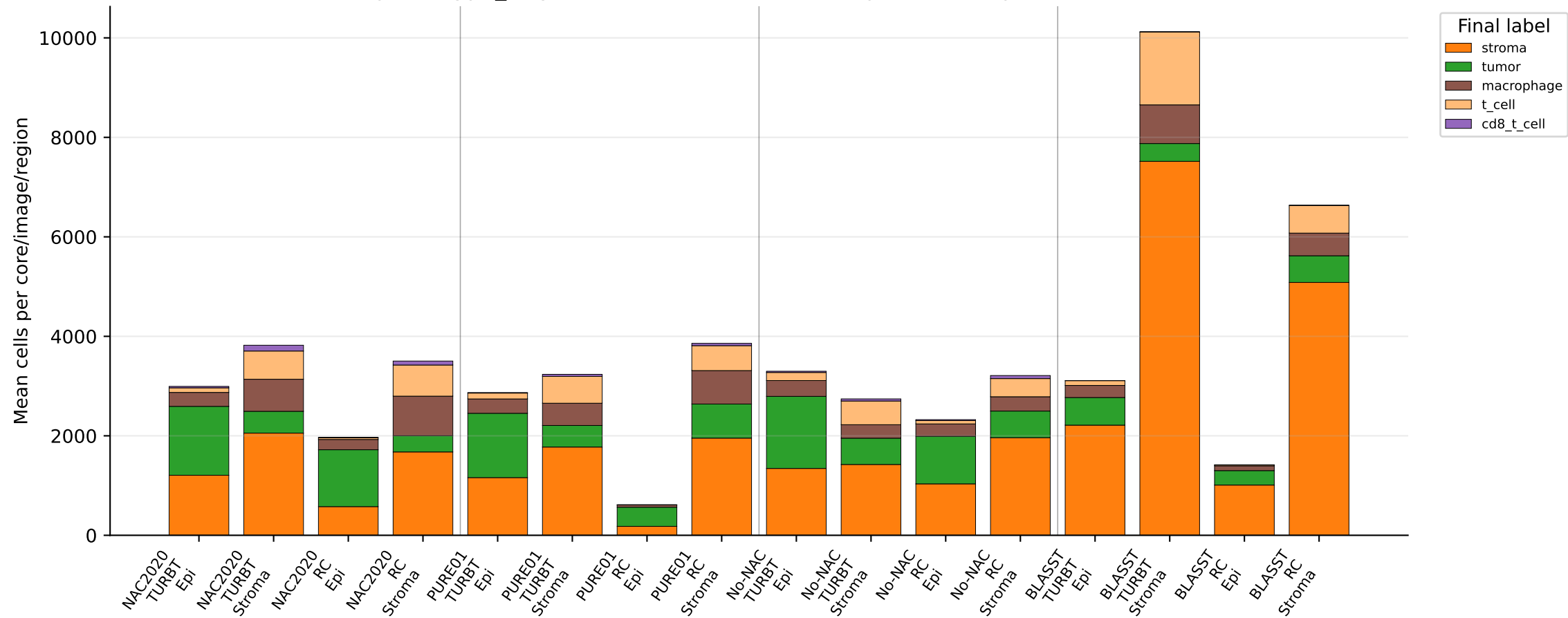
phenotype_only — AR: mean cell-count composition in Epi vs Stroma
