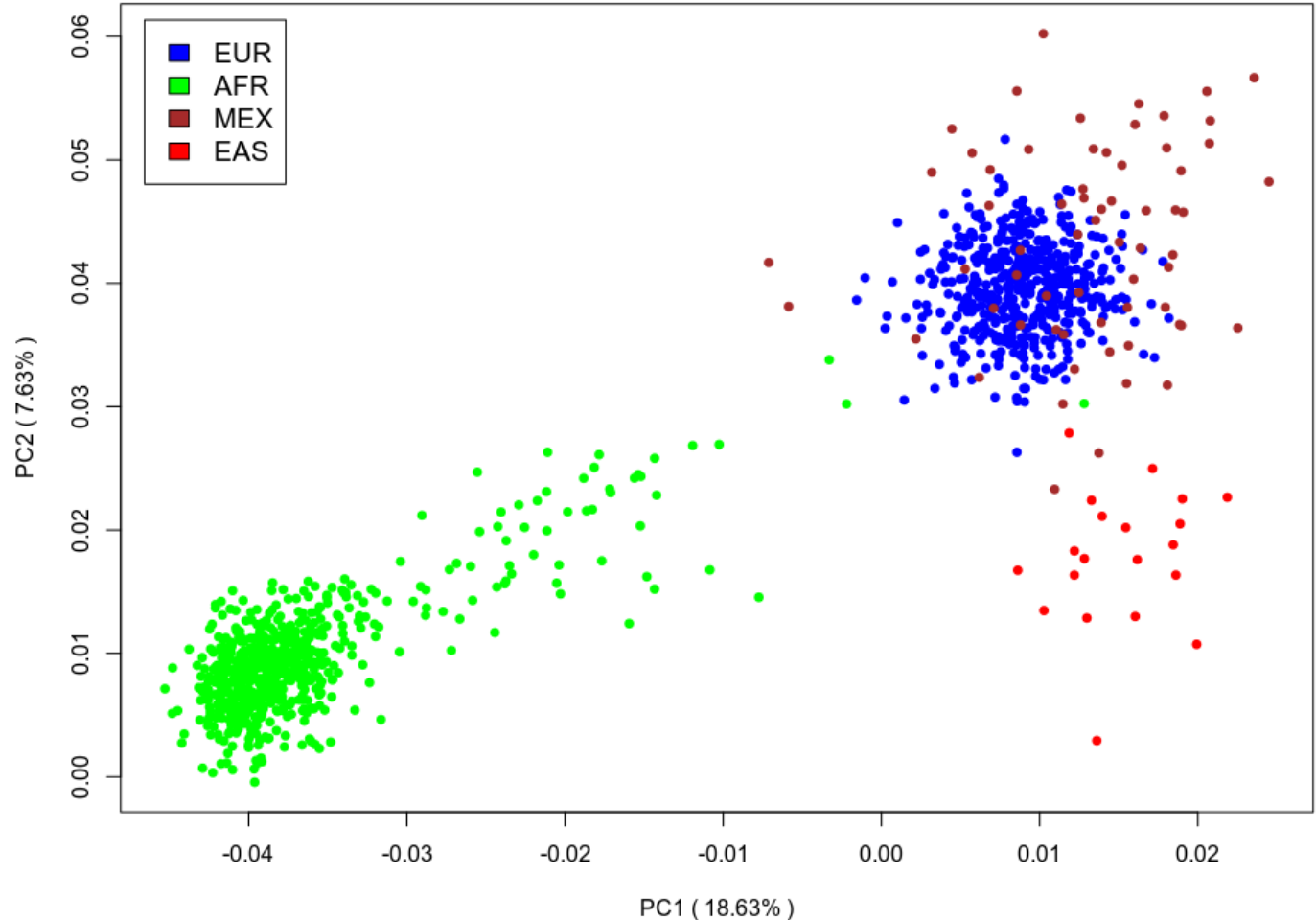
1000G: PCA covariance matrix corrected for uneven population size
