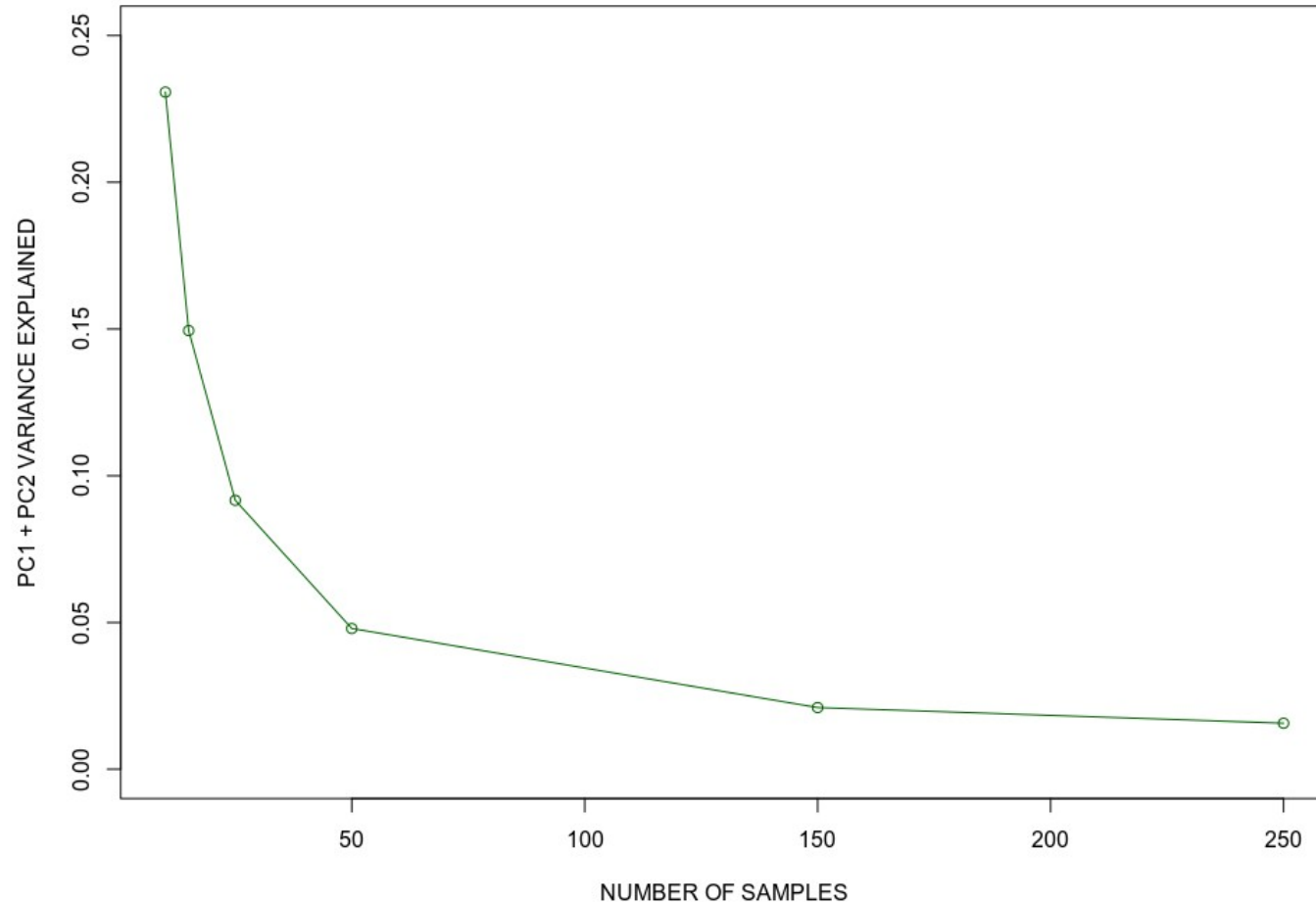
1000G_EUR: EFFECT OF NUMBER OF SAMPLES ON VARIANCE EXPLAINED
