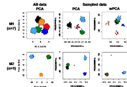
Figure 1. PCA and wPCA projections of simulated
