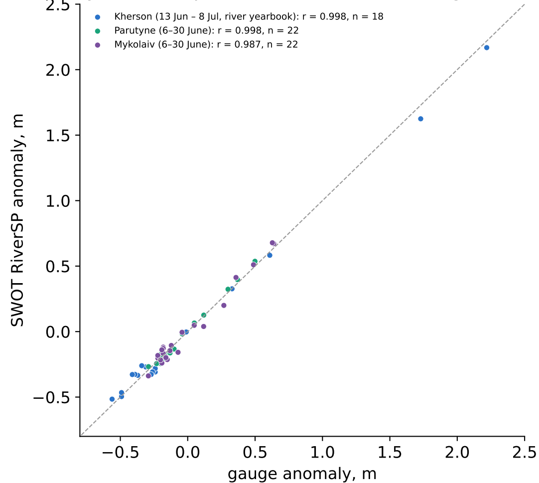
(c) Daily SWOT at posts below the dam through the breach
