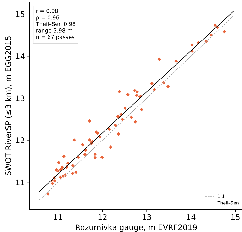
(b) SWOT at Rozumivka after the breach, Aug 2023 – Apr 2025
