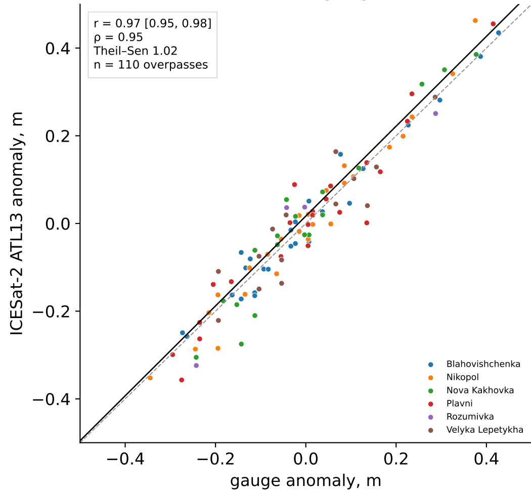
(a) ATL13 at the six reservoir gauges, before the breach
