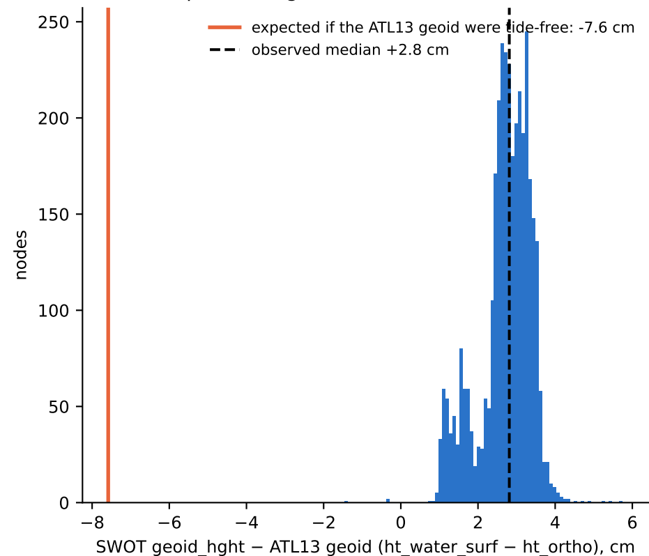
(a) the two products' geoids at the same nodes ( n = 3483 )
