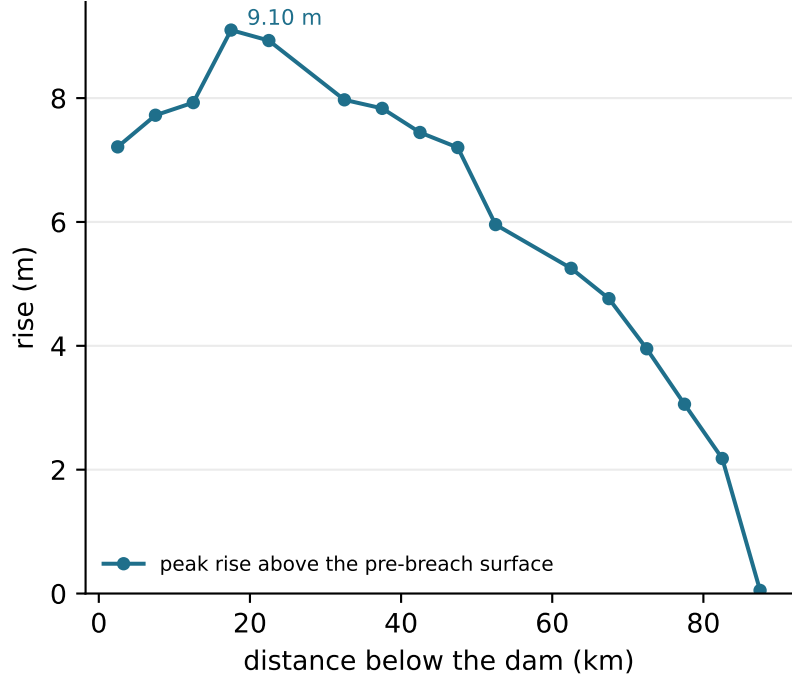
b · the wave, decaying downstream
