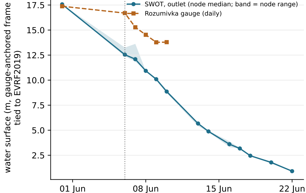
a · the pool emptying, outlet vs upstream gauge
