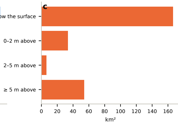
C S1-only (261 km 2 ) by ground elevation vs surface (173 km 2 normally wet; \geq 5 m = false SAR water, ICESat-2 Fig08)
