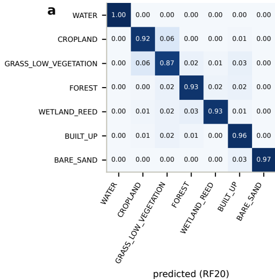
row-normalised confusion, spatial-block CV (rev 2)
