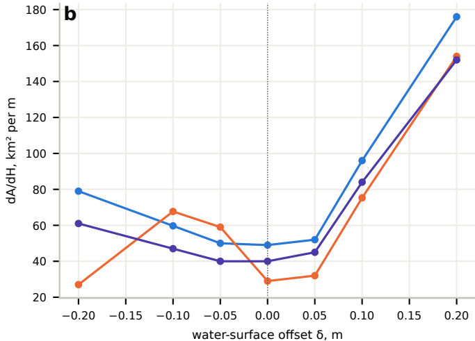
Connectivity thresholds: the reconstructed area under a uniform water-surface offset on the nominal terrain (a sensitivity, not a model)
