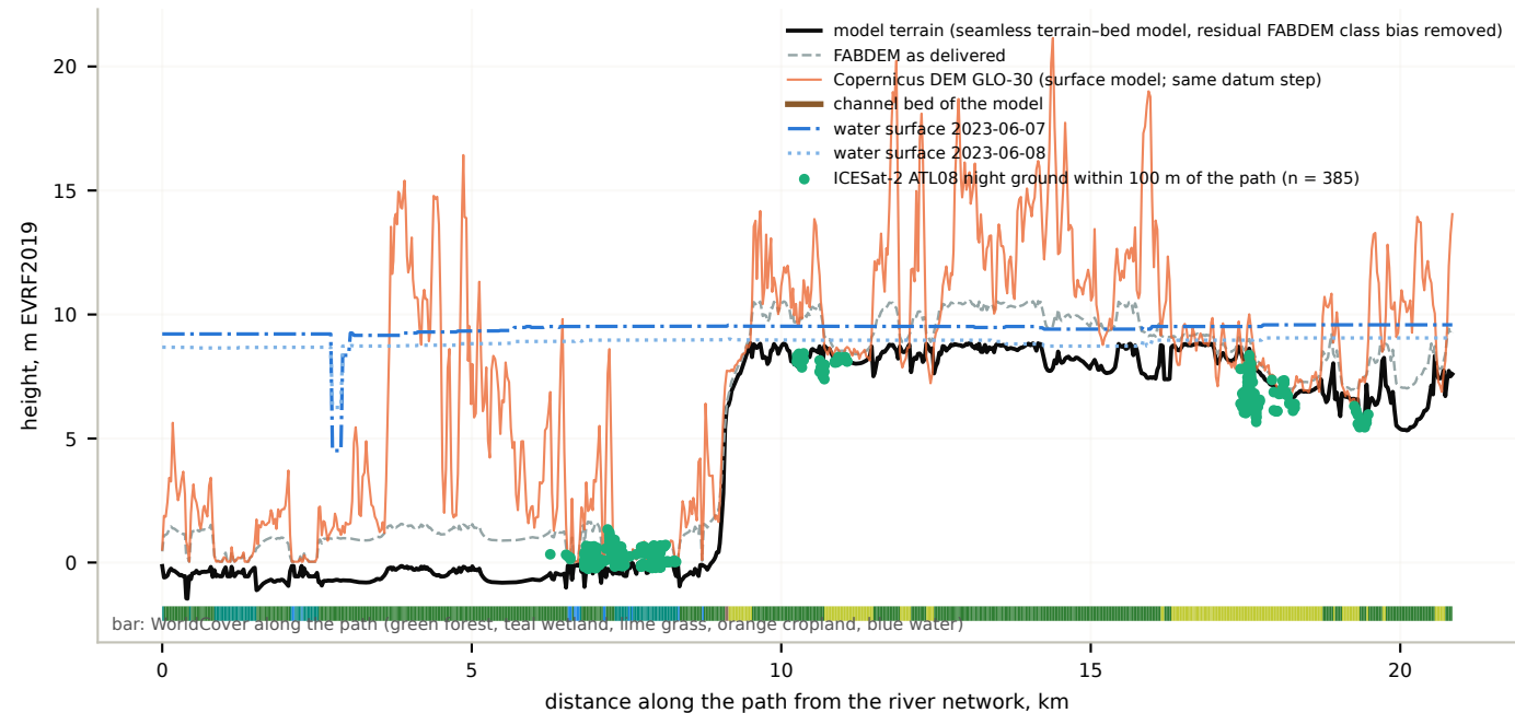
Lowest path from the river network to the floodplain lowland south of Krynky: saddle 8.85 m; head at the saddle 06-07 +0.68 m, 06-08 +0.13 m
