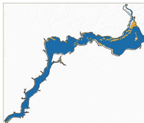
(g) S1 06-13 1938 km 2 dark, IoU 0.85
