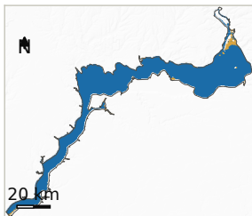
(e) S1 06-01 1964 km 2 dark, IoU 0.98
