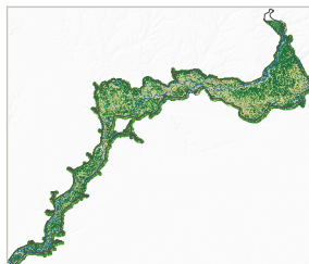
(k) S2 classes 09-08 99% observed
