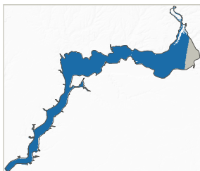
(i) S2 classes 06-05 99% observed
