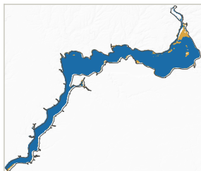
(f) S1 06-08 1705 km 2 dark, IoU 0.97
