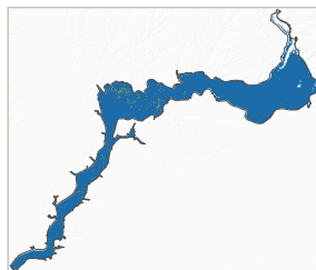
(l) S2 water 06-20 648 km 2
