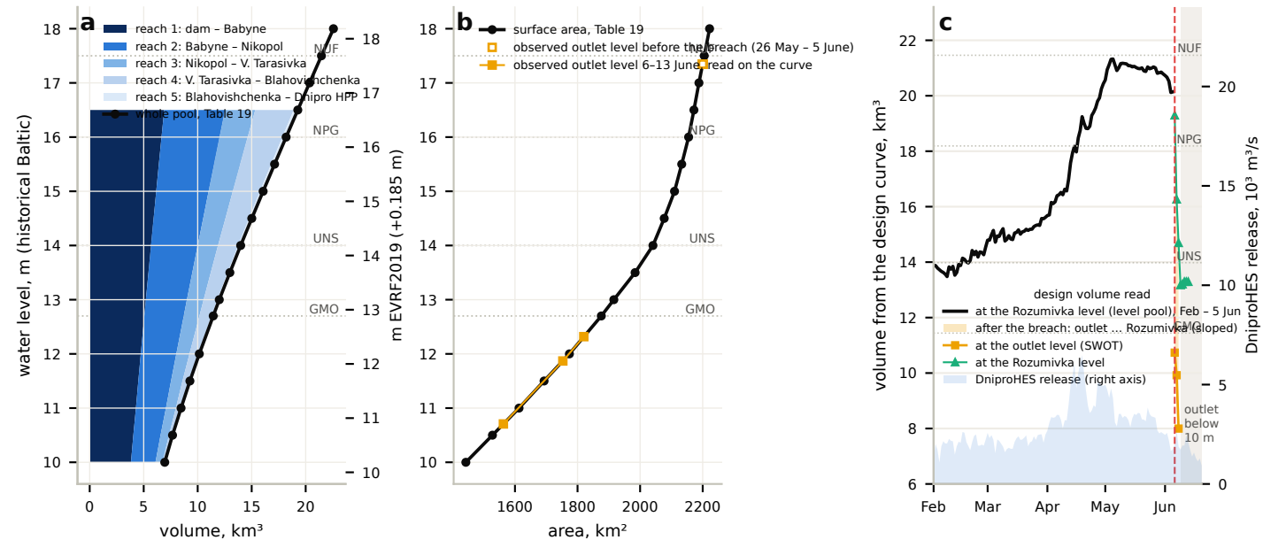
Kakhovka reservoir design hypsometry (monograph Table 19 / Figs 13–15) and the observed 2023 levels read on it — no DEM, nothing fitted
