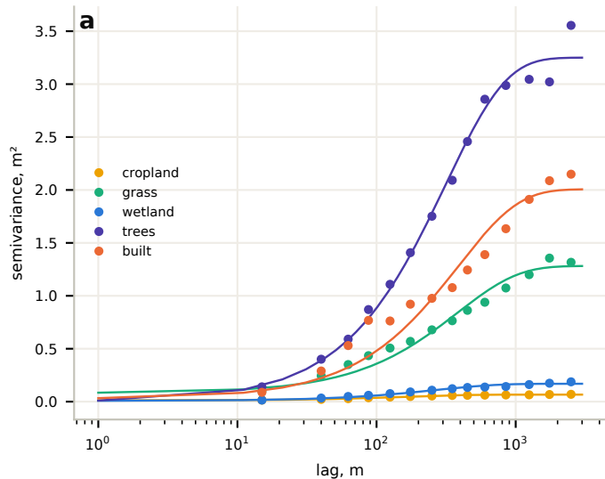
FABDEM – ICESat-2 residual after the class median (pooled)
