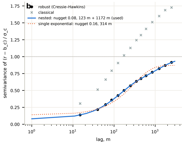
standardized residual: the correlation model of the terrain field
