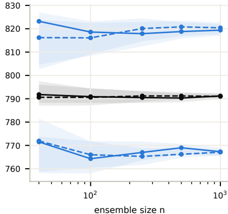
total water-surface area, km 2 , 7 June
