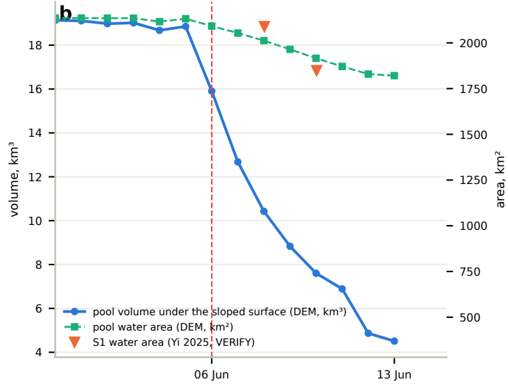
Reservoir drawdown and the downstream flood: levels, pool area/volume, daily balance and the hypsometry used
