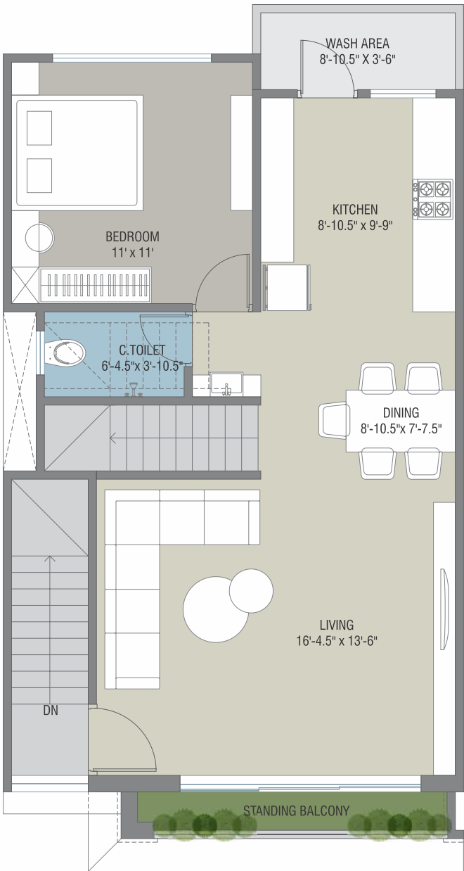
First Floor
